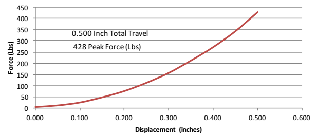
EXAMPLE B Urethane Elliptical PAC-BR101- Orange
