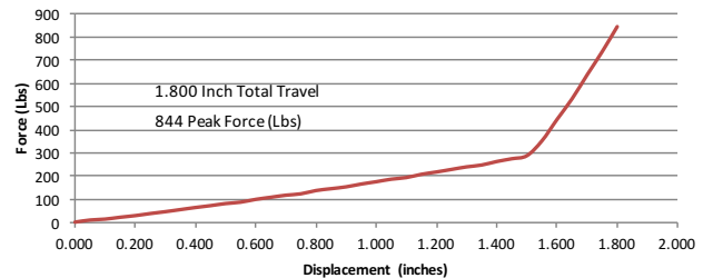
EXAMPLE C Bump Spring Stack PAC-B2x1.190x200 Over PAC-B1x1.70x2000
